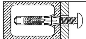
Install anchor.
